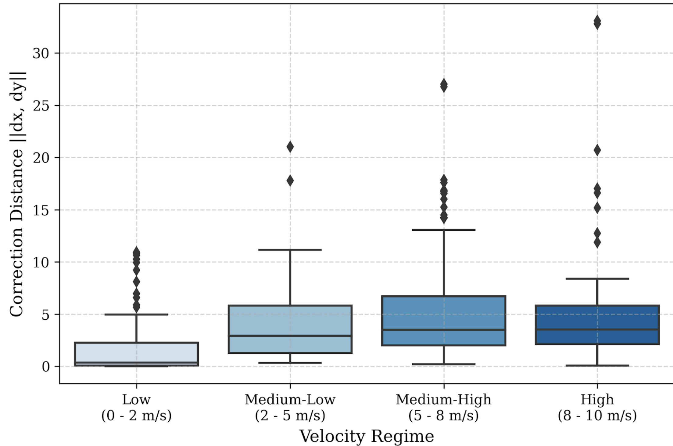
Distribution of EKF Corrections Across Velocity Regimes
